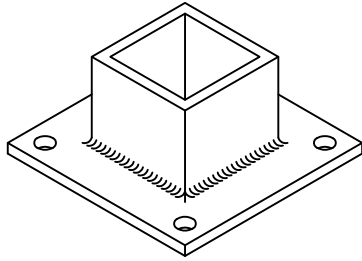
WELDED BASE PLATE PREPUNCHED HOLES FOR ANCHORS 2" SQ. POST
