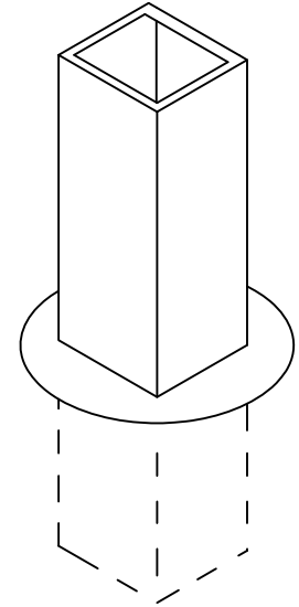
CORE DRILLED HOLE POST SET IN GROUT 2" SQ. POST
